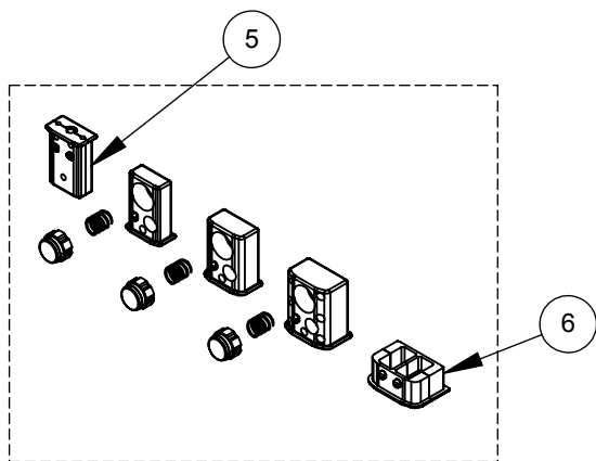
91501 COMPLETE LOCK SET
